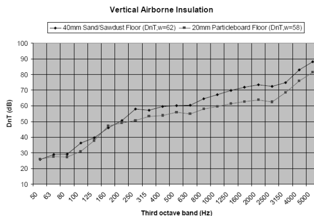
Figure 11. Vertical airborne sound insulation measurements.
