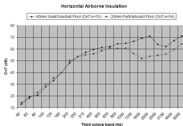
Figure 10. Horizontal airborne sound insulation measurements.
