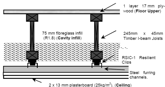
Figure 7. The basic subfloor used for the flanking transmission measurements.
