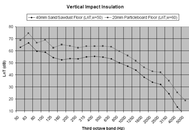
Figure 9. Vertical impact sound insulation measurements.
