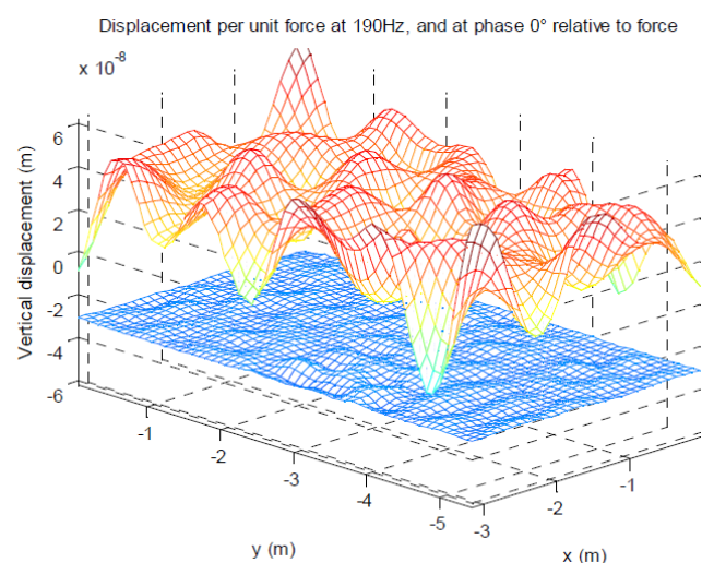
Figure 5. Measured vibration (displacement) of a Floating Gypsum Concrete floor upper surface and ceiling from 1N of forced vibration on the upper surface.
