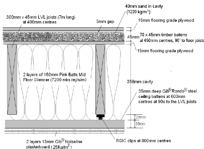
Figure 13. The ‘40mm Sand Floor’.
